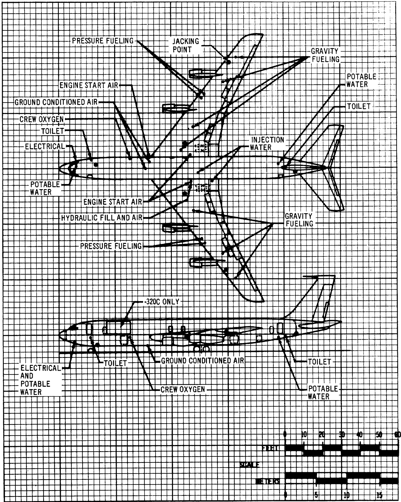
GROUND SERVICE CONNECTIONS MODELS 707-320, -320B, -320C, -420
