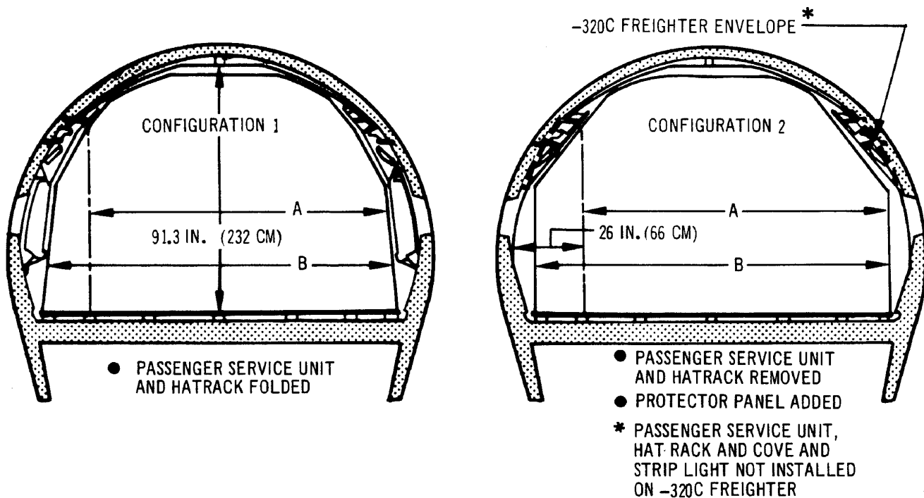
PALLET ENVELOPES BASED ON 1-INCH MINIMUM CLEARANCE (PALLETS 2 THRU 12)
