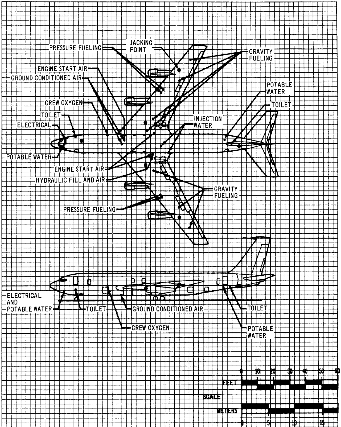
5.4 GROUND SERVICE CONNECTIONS MODEL 707-120B
