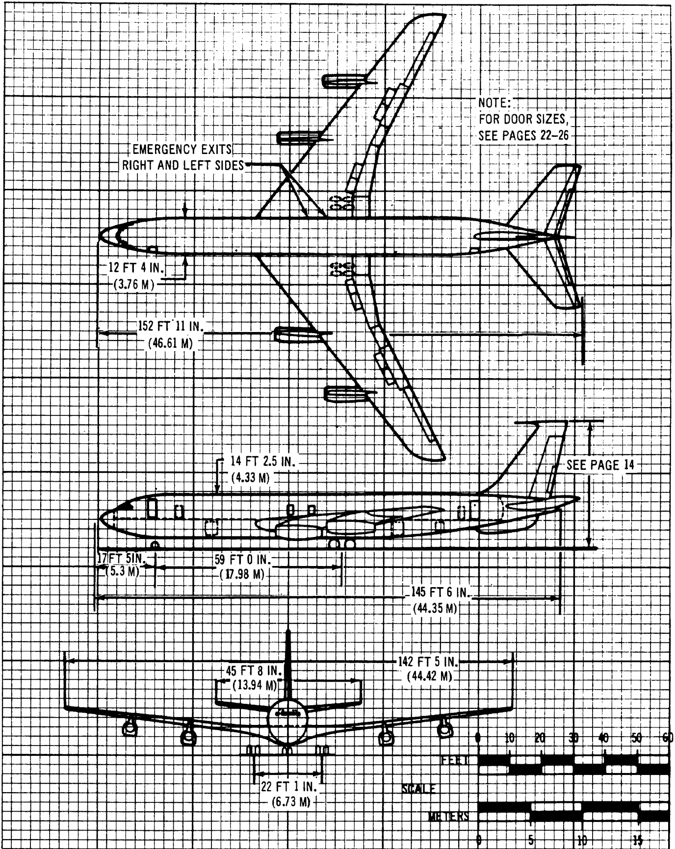
GENERAL DIMENSIONS MODELS 707-320, -420
