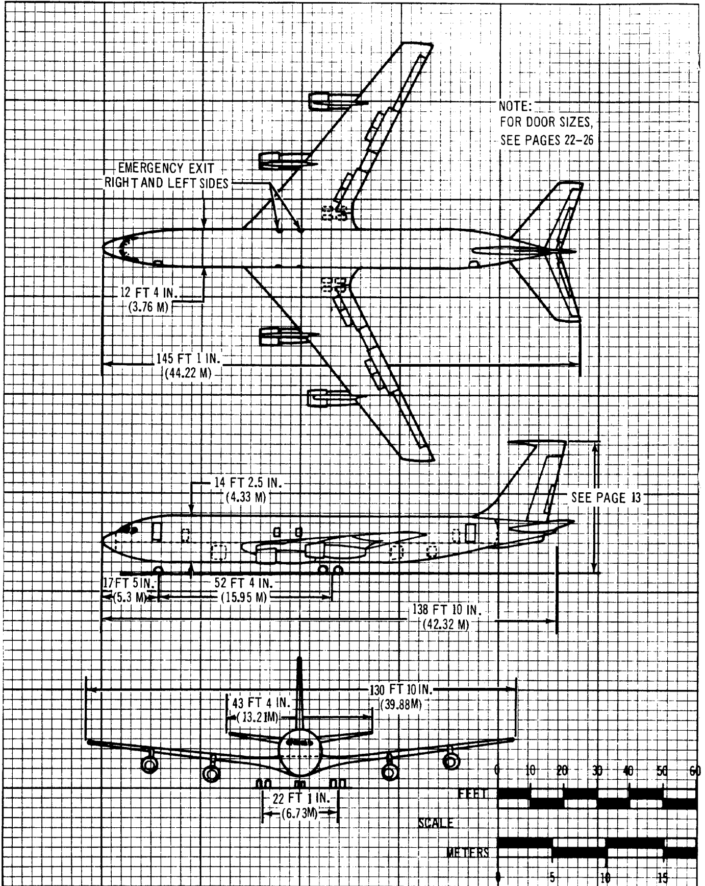
2.2 GENERAL DIMENSIONS MODEL 707-120B
