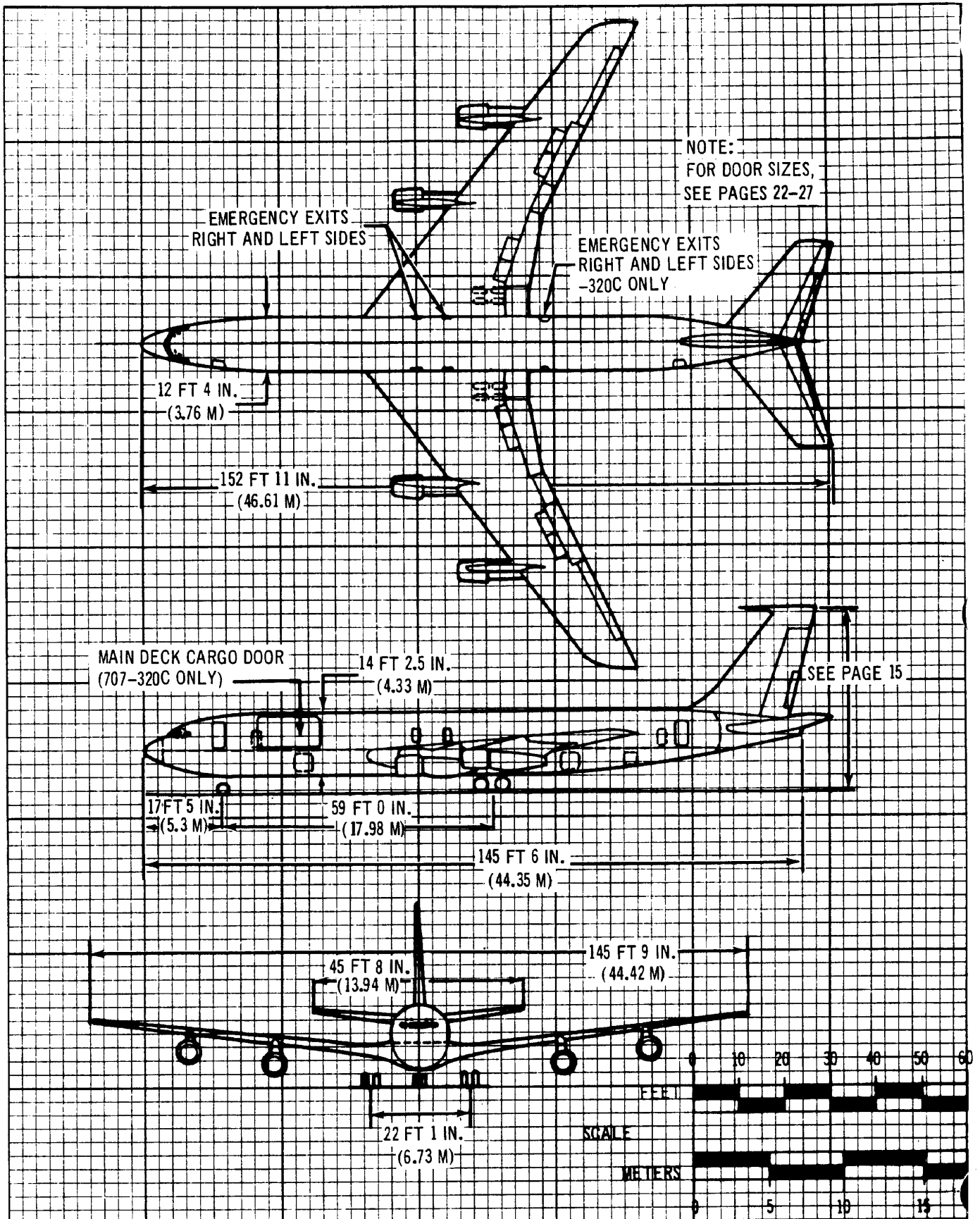
GENERAL DIMENSIONS MODELS 707-320B, -320C
