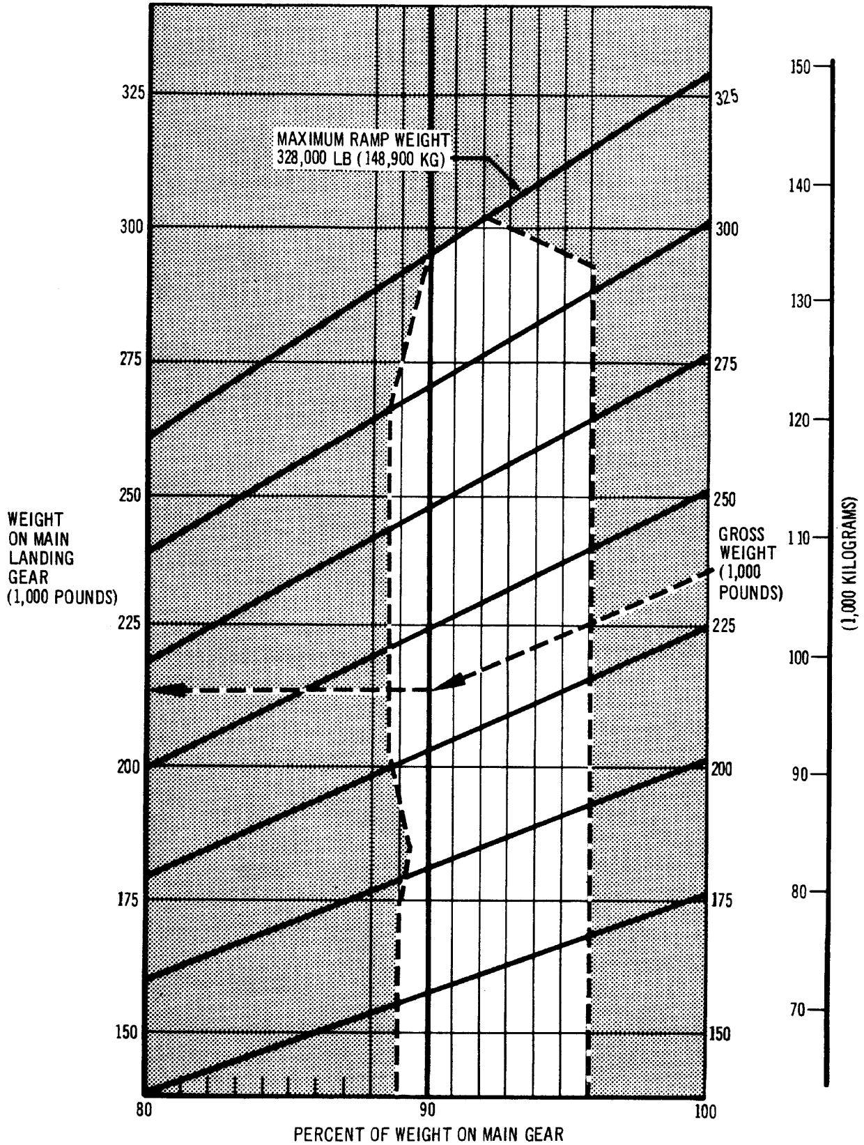
LANDING GEAR LOADING ON PAVEMENT MODEL 707-320B
