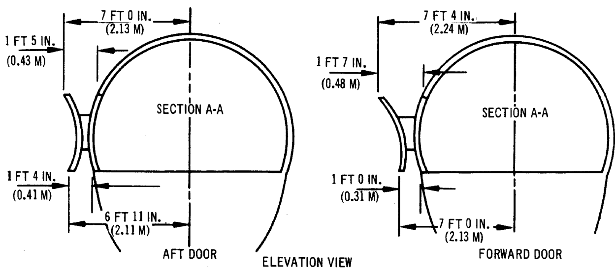
DOOR CLEARANCES - FORWARD AND AFT GALLEY SERVICE MODELS 707-120B, -320, -320B, -320C, -420
