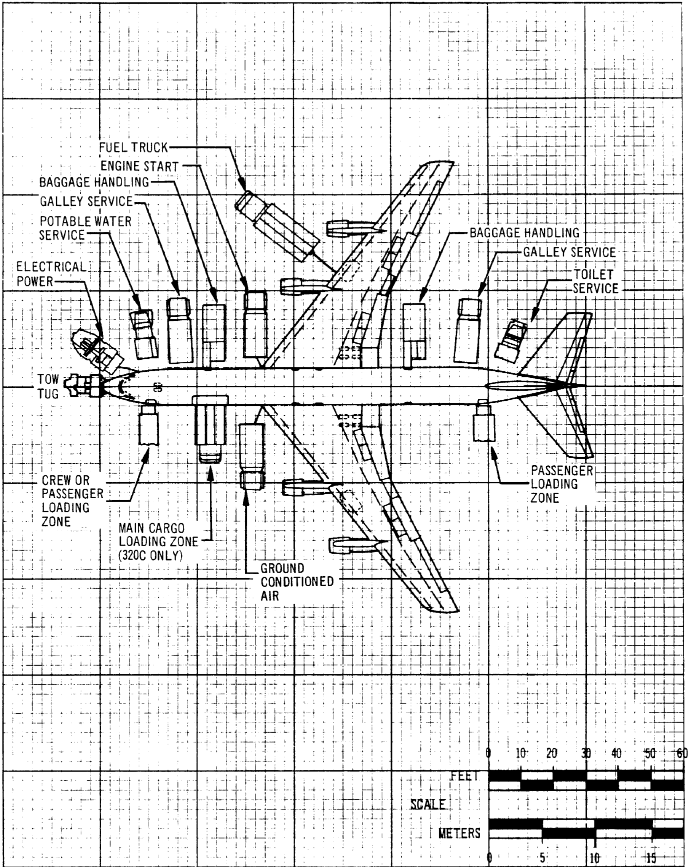
AIRPLANE SERVICING ARRANGEMENT (TYPICAL) MODELS 707-320, -320B, -320C, -420
