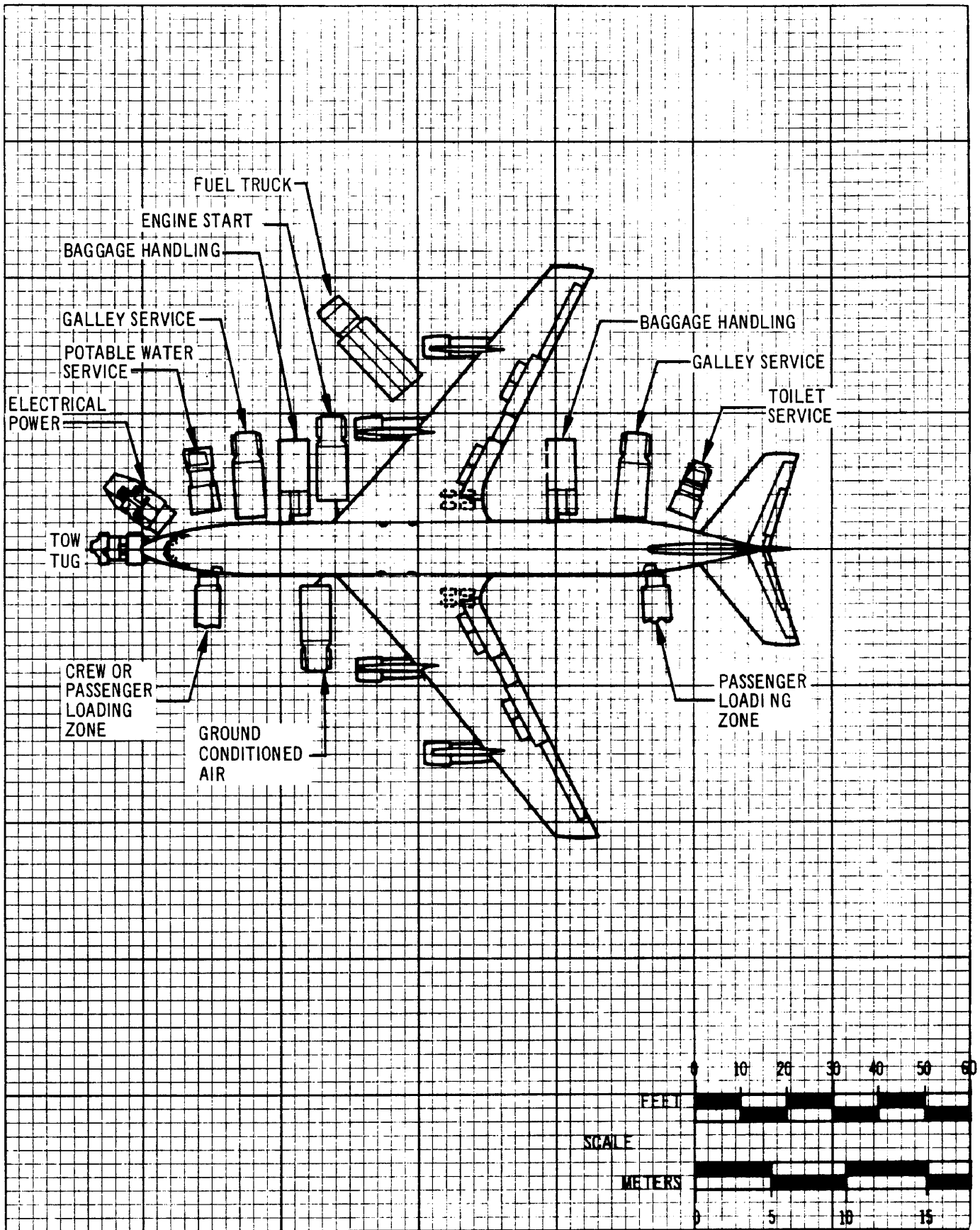
5.1 AIRPLANE SERVICING ARRANGEMENT (TYPICAL) MODEL 707-120B
