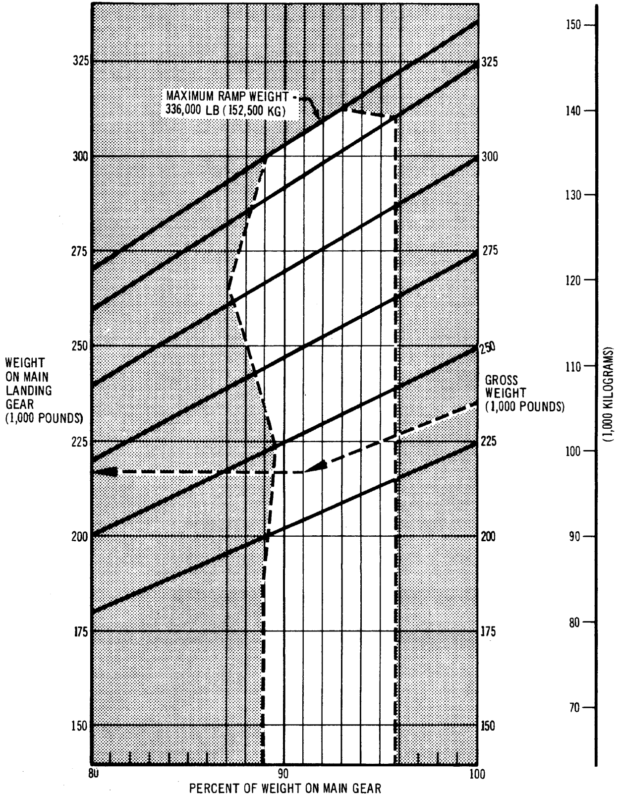
LANDING GEAR LOADING ON PAVEMENT MODEL 707-320C
