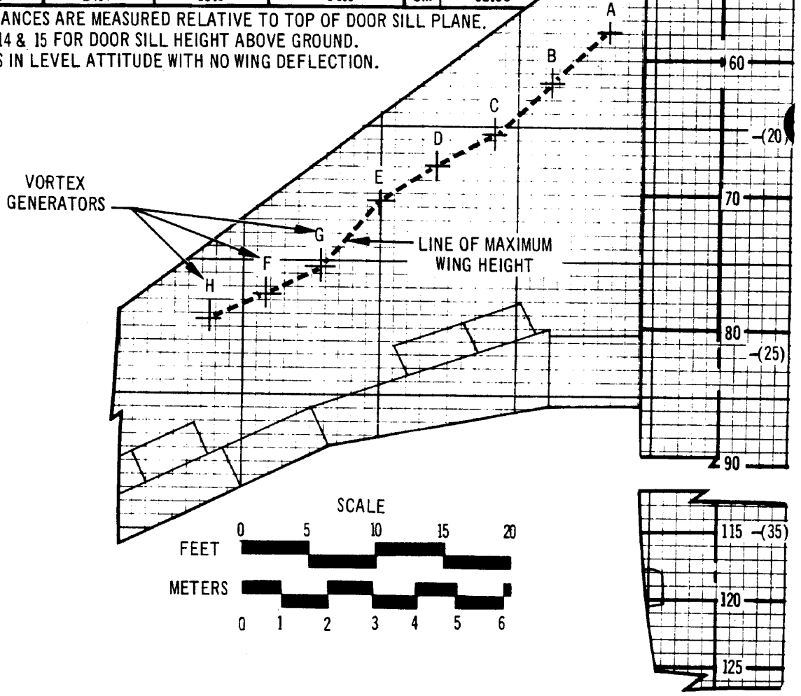
DOOR SILL/WING CLEARANCE — CRITICAL INTERFERENCE PATH MODEL 707-320, -320B, -320C, -420
