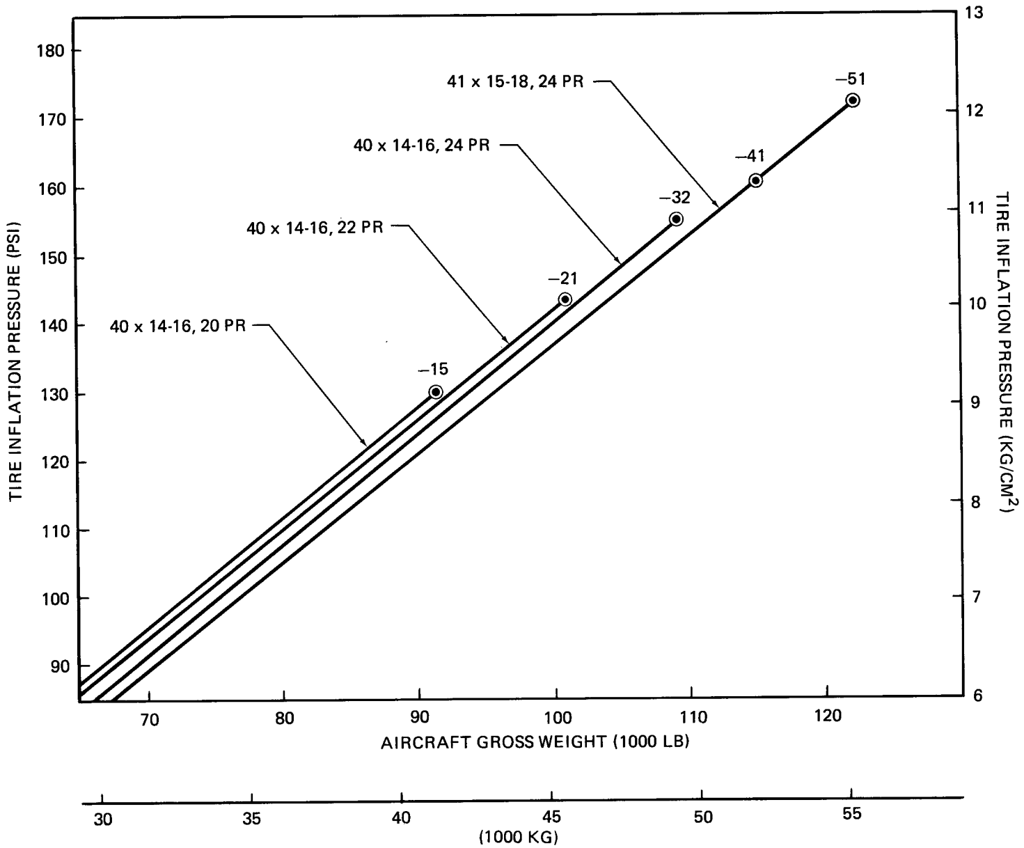
7.2.1 TIRE INFLATION CHART – MODELS DC-9-15, -21, -32, -41, -51
