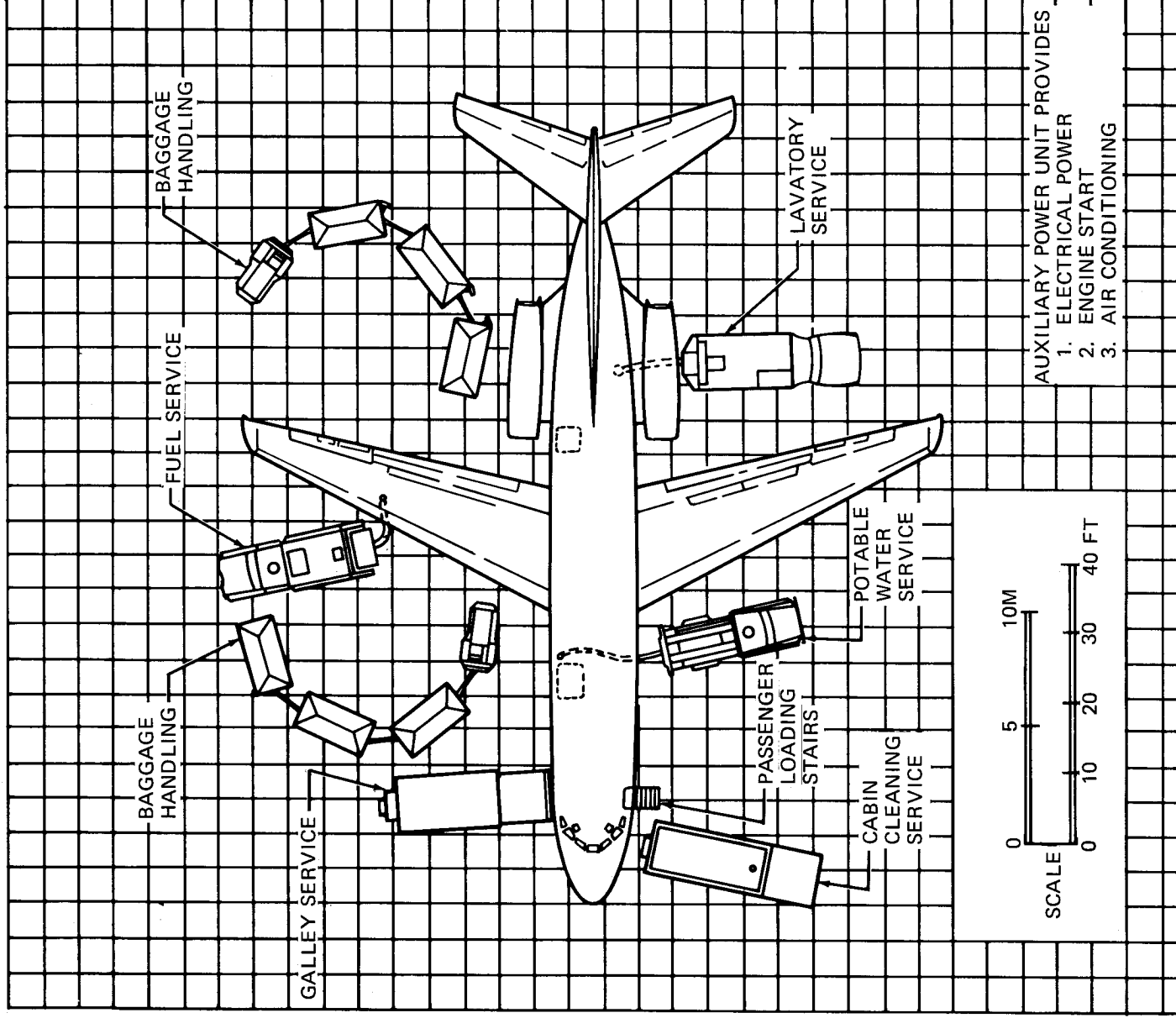
5.1 AIRPLANE SERVICING ARRANGEMENT (TYPICAL) MODEL DC-9-21
