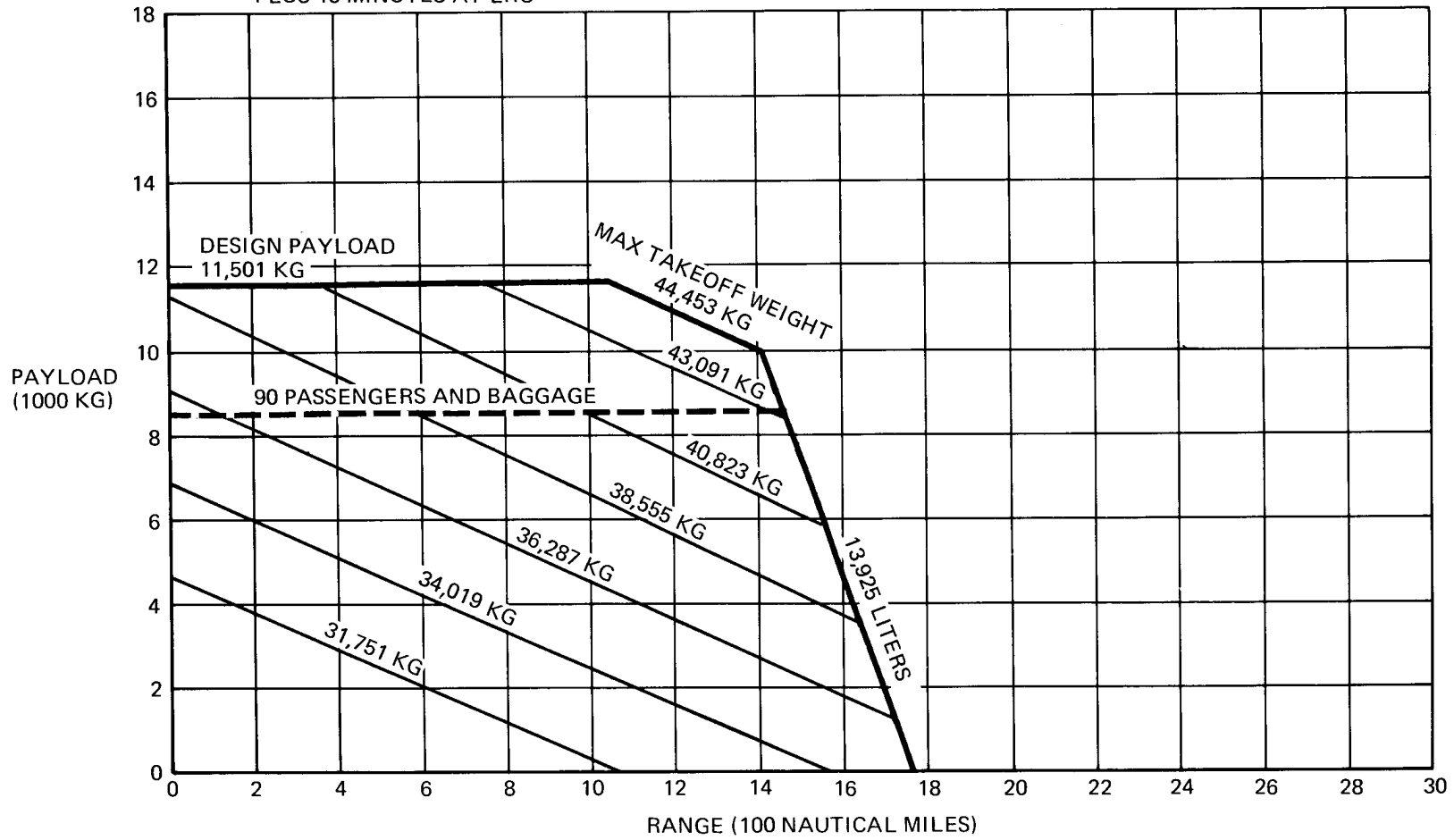
3.2 PAYLOAD-RANGE PAYLOAD-RANGE FOR TYPICAL LONG-RANGE CRUISE AT 9150 METERS MODEL DC-9-21
