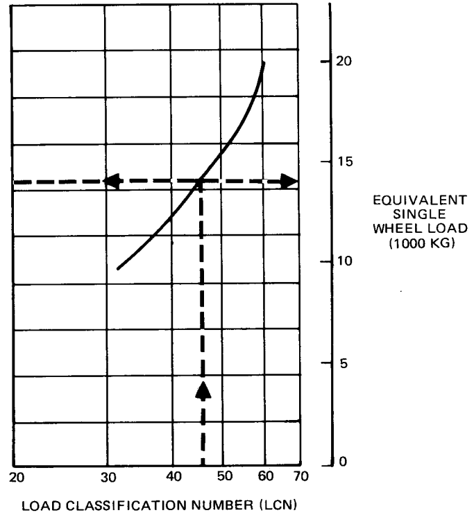
40 x 14 TIRES – TIRE PRESSURE CONSTANT AT 155 PSI (10.9 KG/CM 2 )
