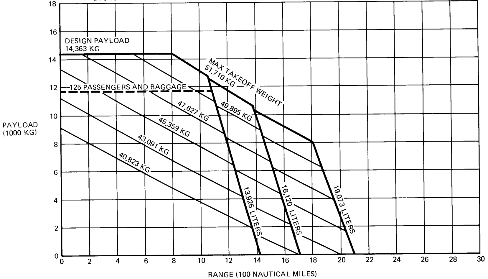
3.2 PAYLOAD-RANGE PAYLOAD-RANGE FOR TYPICAL LONG-RANGE CRUISE AT 9,150 METERS MODEL DC-9-41
