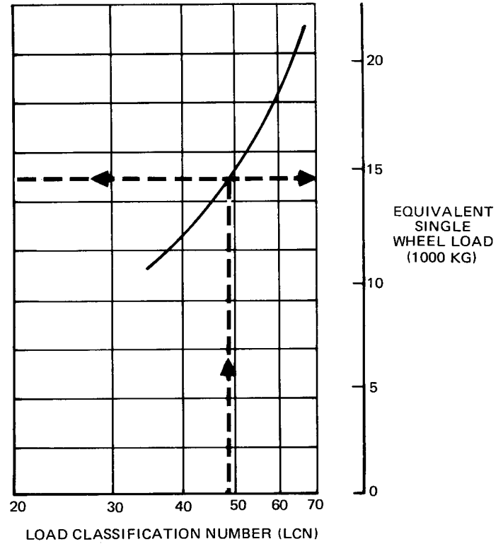
41 x 15 TIRES – TIRE PRESSURE CONSTANT AT 160 PSI (11.3 KG/CM 2 )
