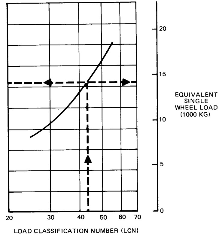
40 x 14 TIRES – TIRE PRESSURE CONSTANT AT 143 PSI (10.1 KG/CM 2 )
