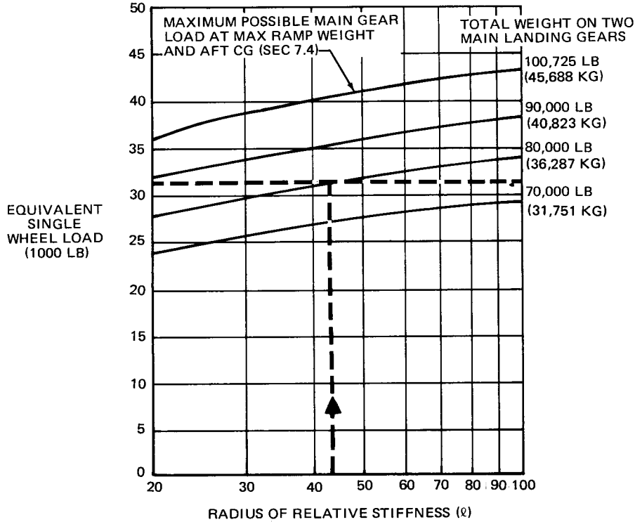
40 x 14 TIRES – TIRE PRESSURE CONSTANT AT 155 PSI (10.9 KG/CM 2 )
