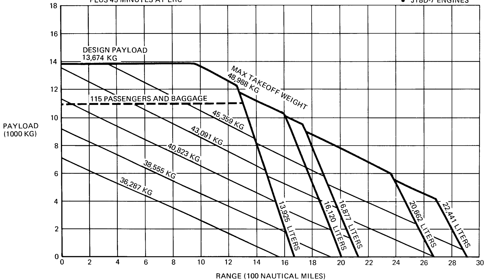
3.2 PAYLOAD-RANGE PAYLOAD-RANGE FOR TYPICAL LONG-RANGE CRUISE AT 9,150 METERS MODEL DC-9-32
