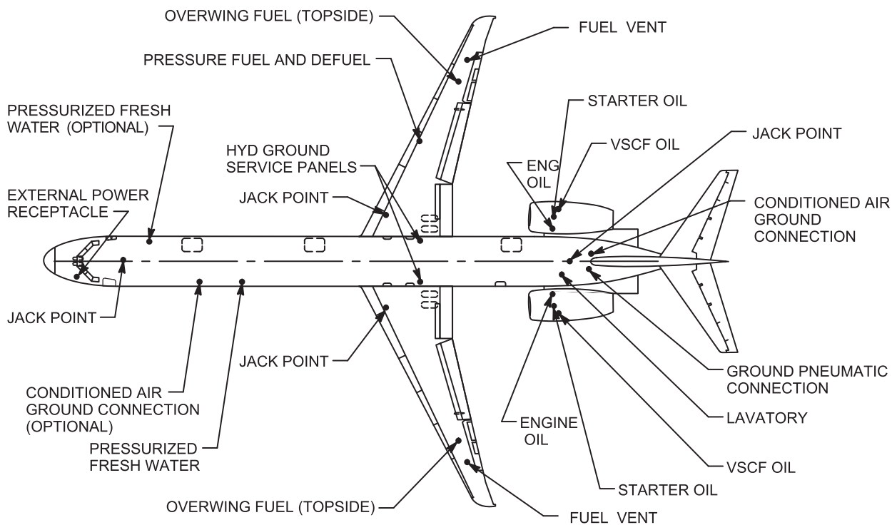
TOP VIEW
