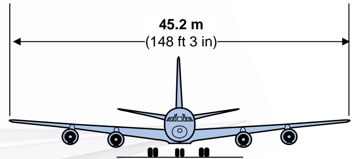
DC-8-62/-63/-72/-73
